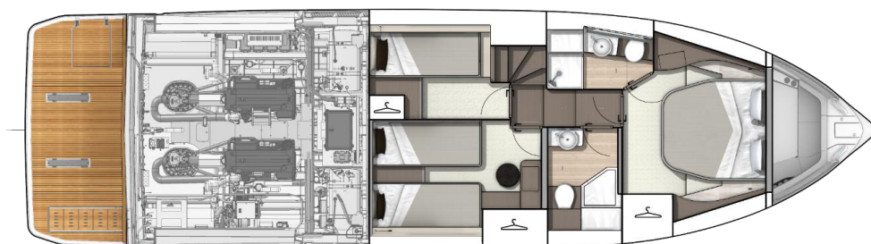
Engine room - Lower deck
